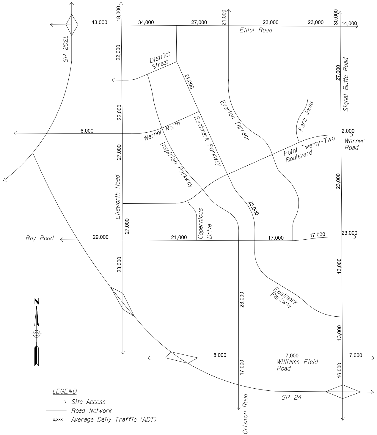
Figure 3.1 MAG Year 2040 Background Traffic Volumes
