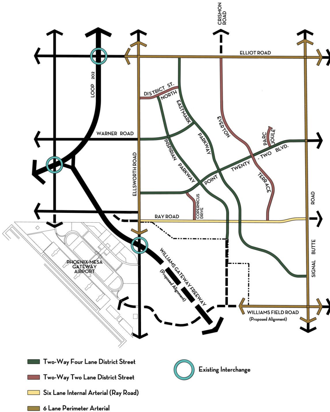
Figure 2.1 Conceptual Master Street Circulation Plan
