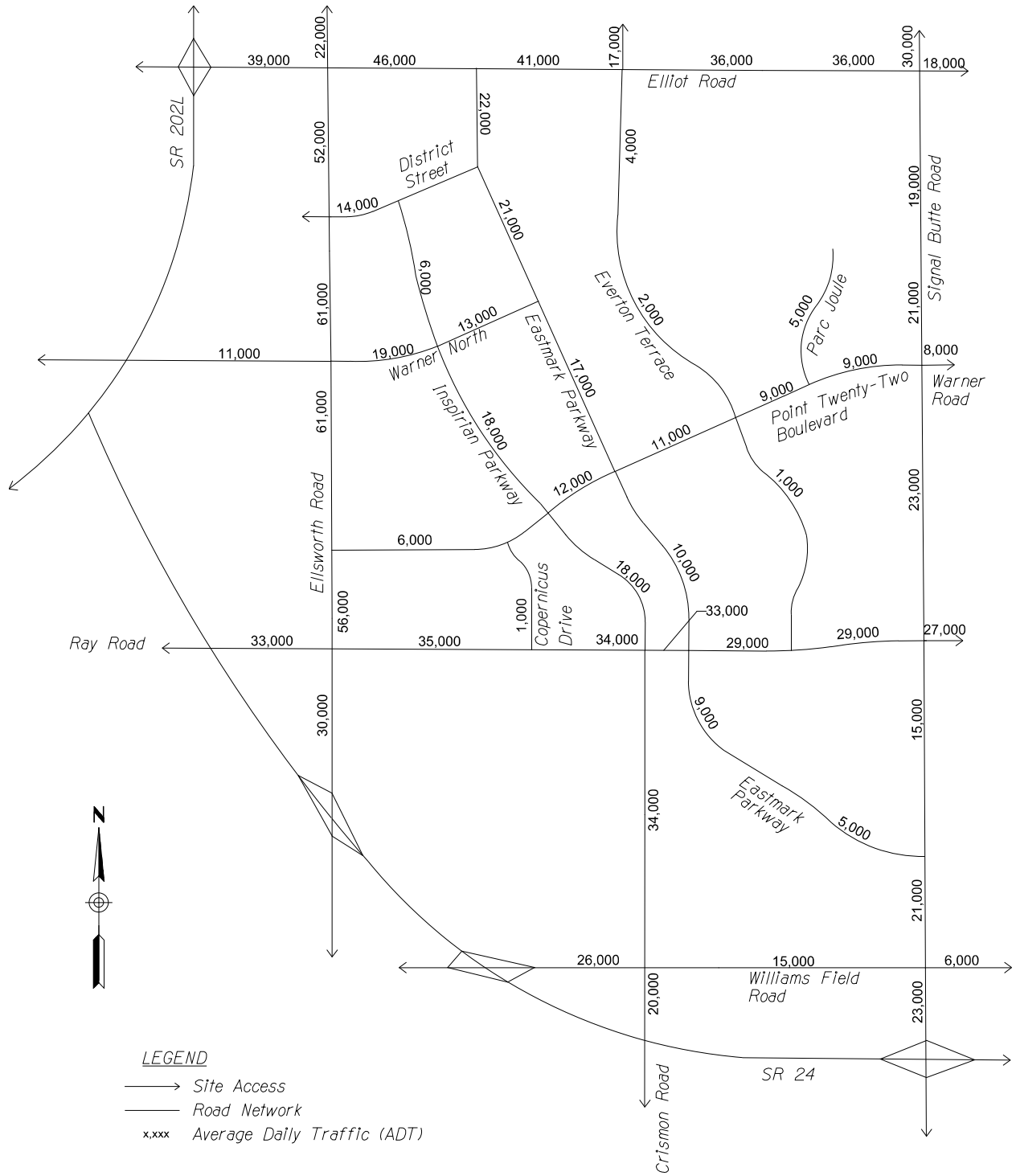
Figure 4.4 Year 2040 Total Traffic for Eastmark – Full Build Out
