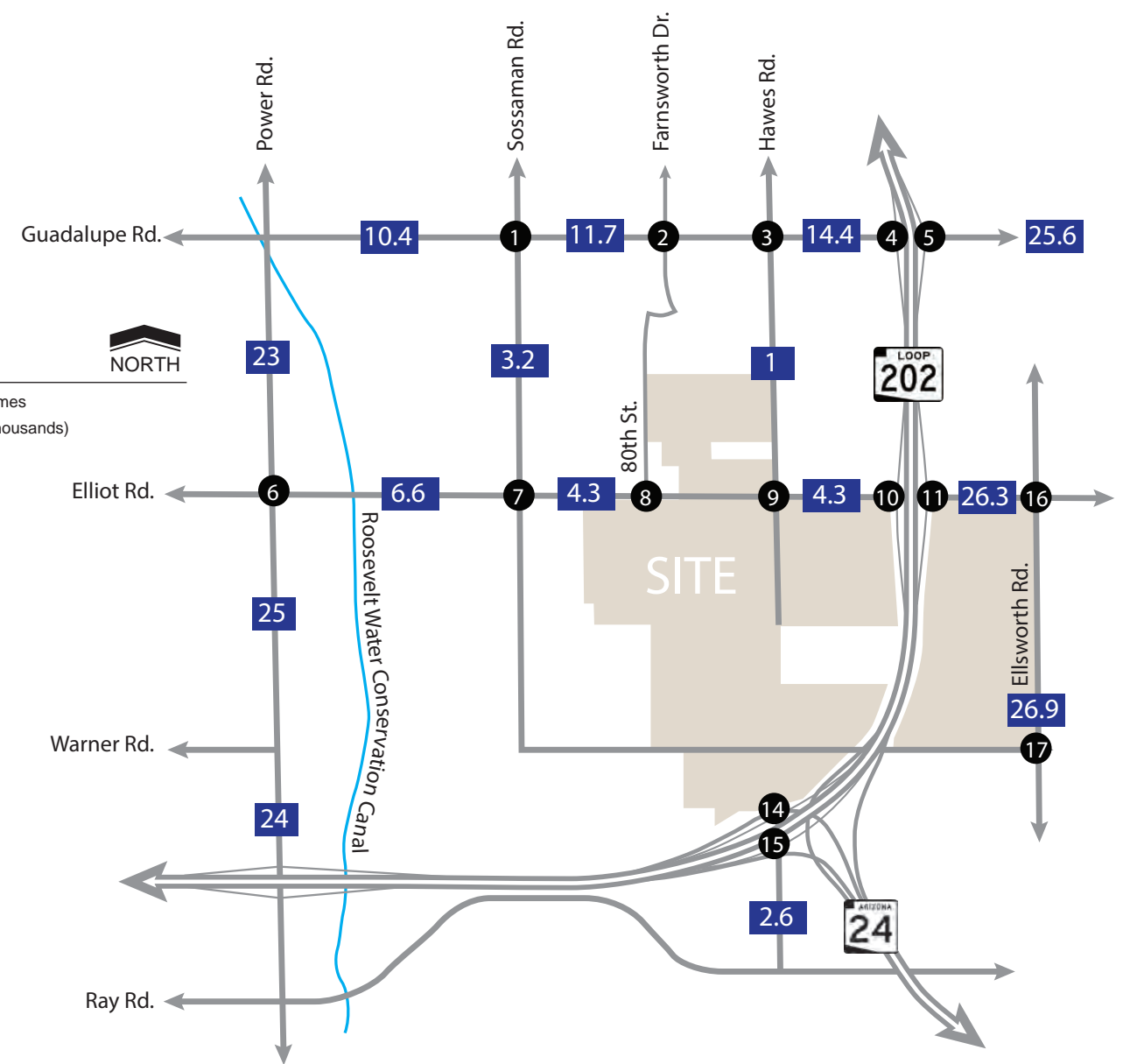
Figure 4: Existing Traffic Volumes
