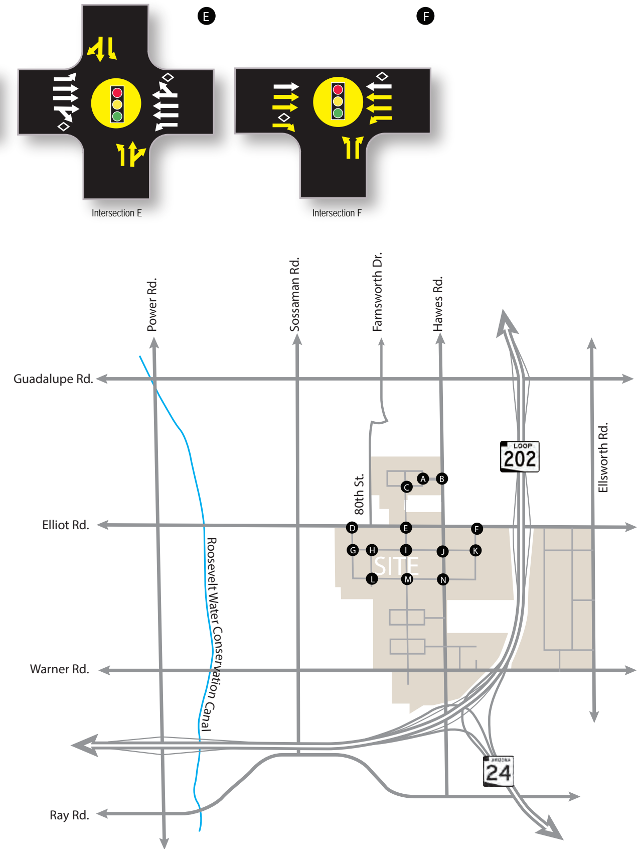
Figure 2I: Proposed Lane Configurations and Traffic Controls B
